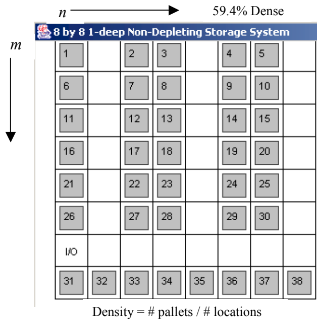
Figure 4 8 by 8, 1-Deep Storage System
