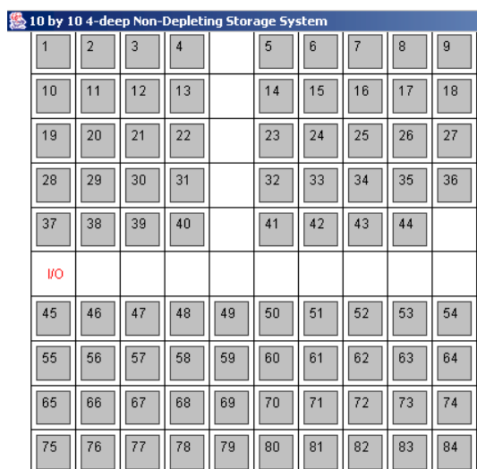
Figure 36 Illustration of a Storage System with an Inverted “T” Design
