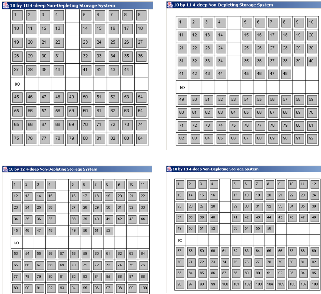
Figure 30 The Ten Best k = 4 Storage Designs, Part 1
