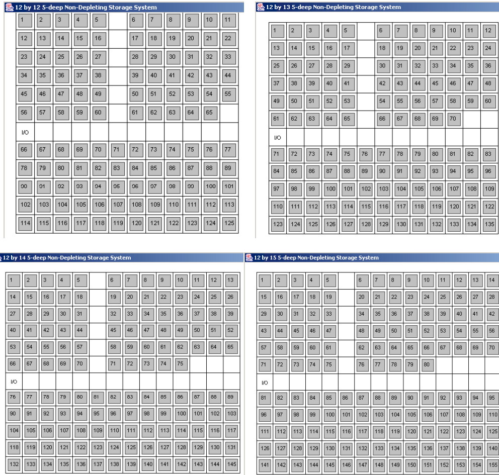
Figure 32 The Ten Best k = 5 Storage Designs, Part 1
