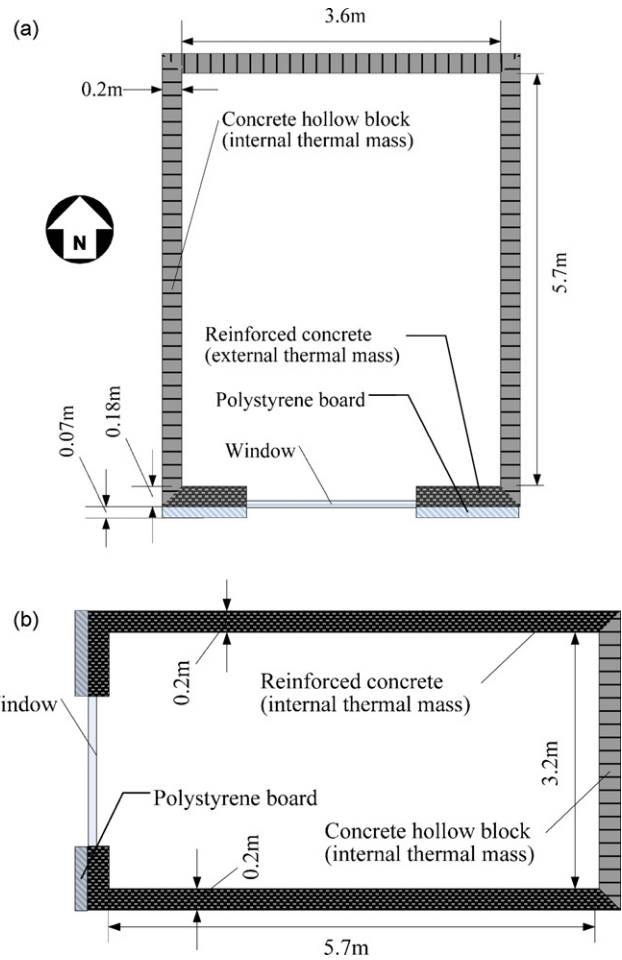
Fig. 5. Schematic of the simulated room: (a) plan view and (b) cross-section view.
