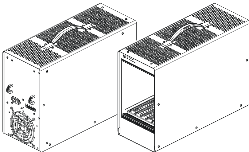
FIGURE 1-7: CT-100C DIMENSIONAL DIAGRAM
