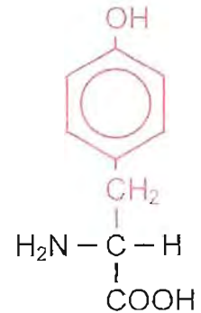
Tirosina (Tyr - Y)
