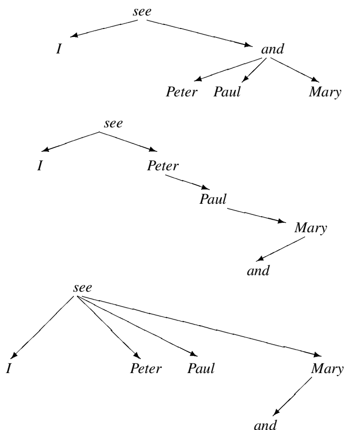
Fig. 5 Three different representations of the structure of (9).
